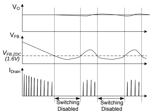
Figure 31. Burst-Mode Operation
