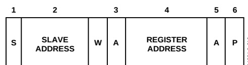
Figure 10. Setting a Register Address for Subsequent Read
