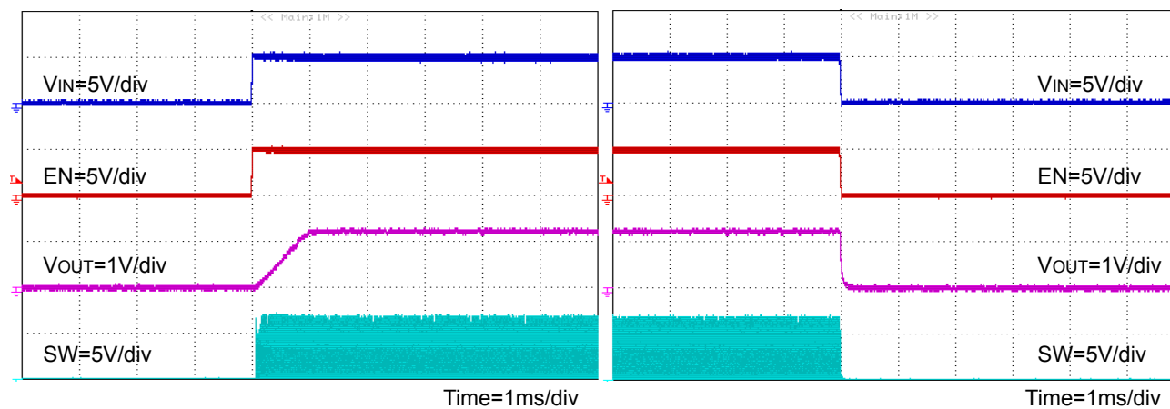
Figure 30. Power Up Waveform with VIN (FREQ=H (1MHz), R_{LOAD}=1.2\Omega )
