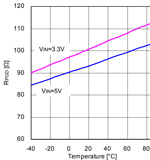
Figure 21. PGD ON ON-Resistance vs Temperature
