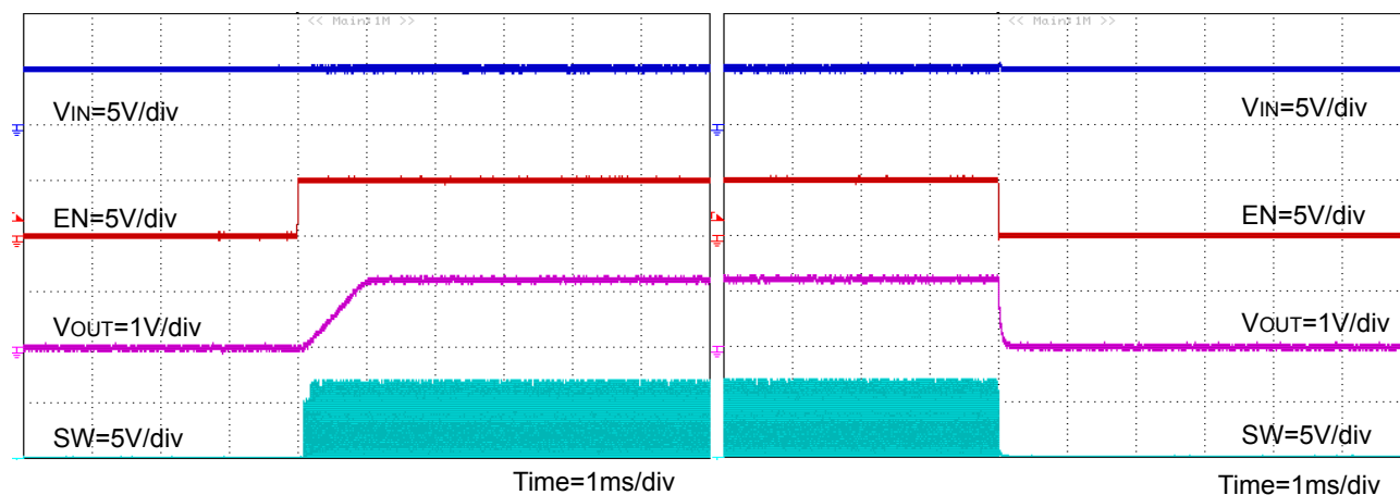
Figure 28. Power Up Waveform with EN (FREQ=H (1MHz), R_{LOAD}=1.2\Omega )
