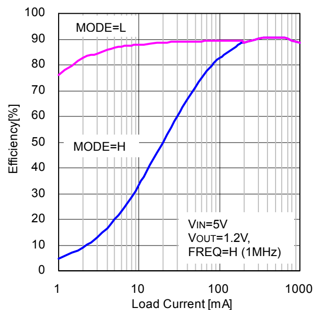
Figure 7. Efficiency vs Load Current
