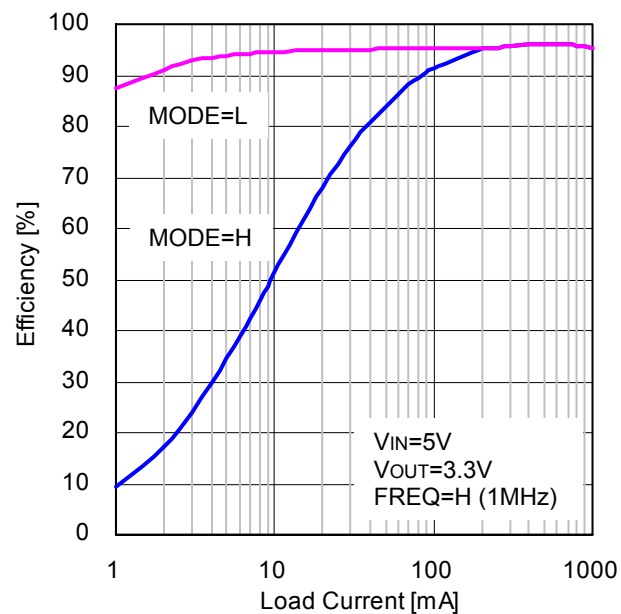
Figure 9. Efficiency vs Load Current
