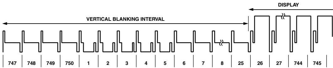
Figure 29. SMPTE296M (720p)
