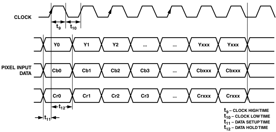
Figure 2. 4:4:4 YCrCb Input Data Format Timing Diagram
