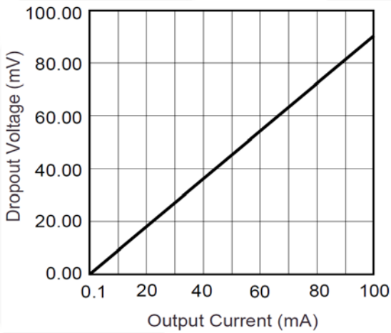
Figure 17. Dropout Voltage
