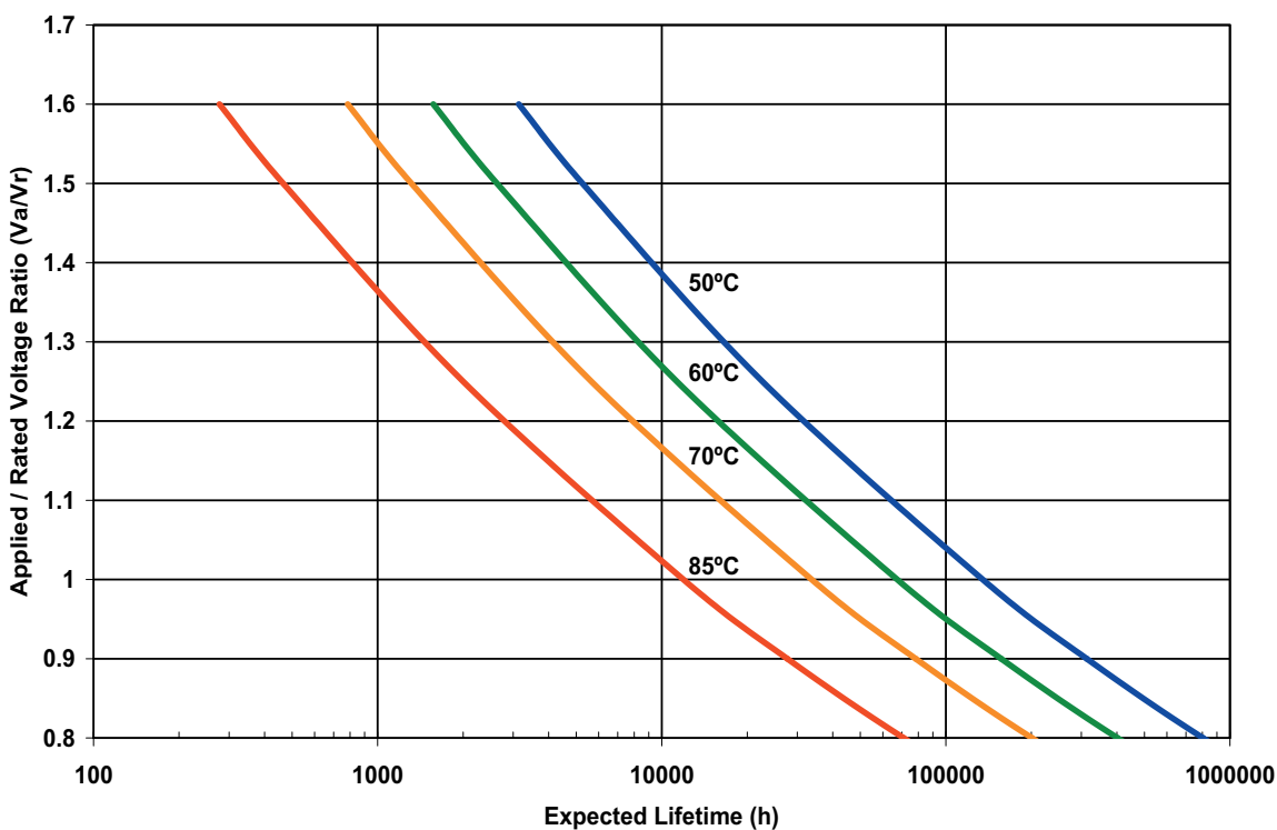
Expected Lifetime vs Applied Voltage and Core Temp
