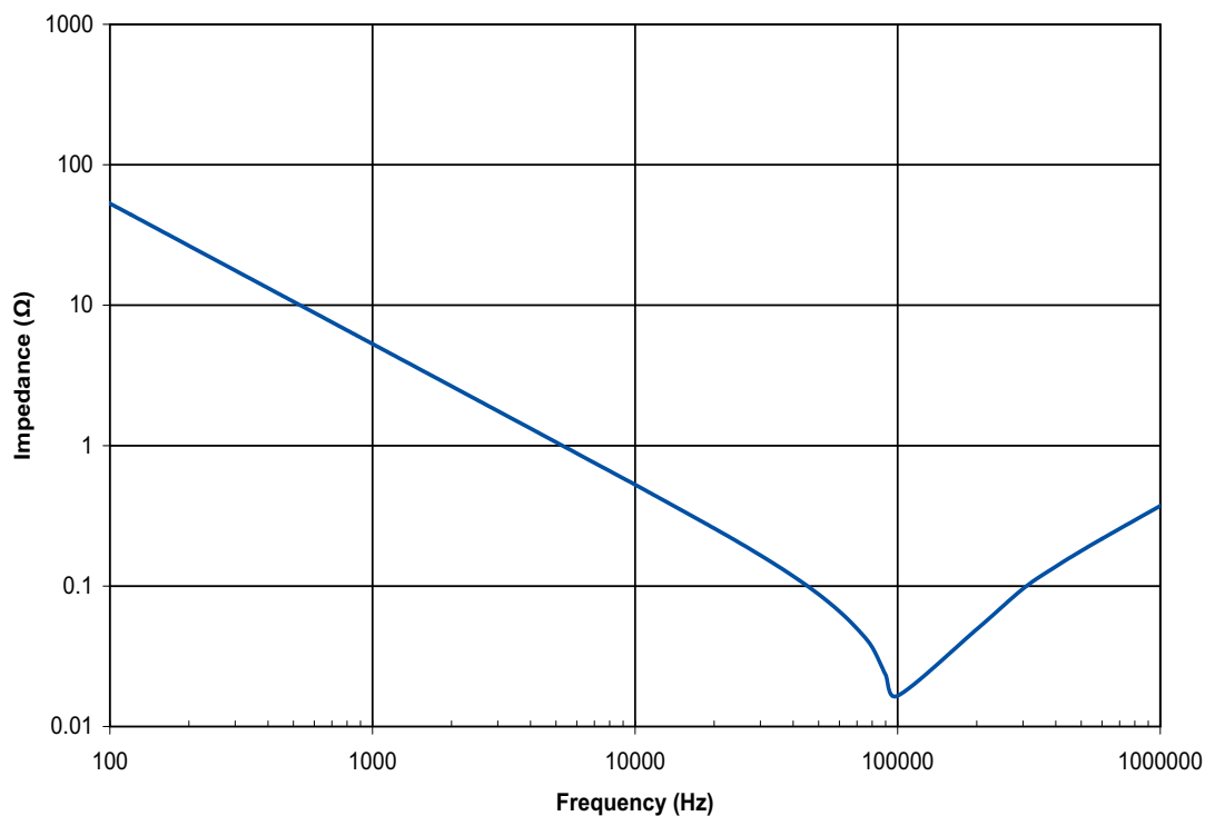
UNL6W30K-F Impedance vs Frequency
