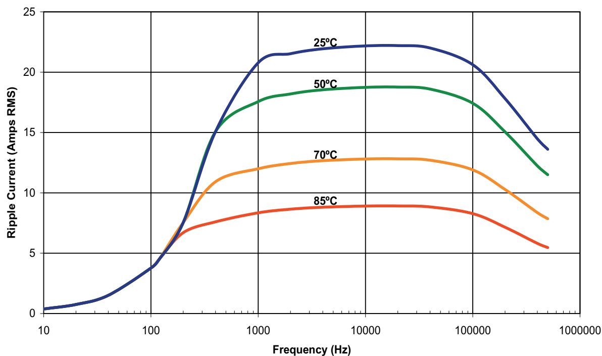
Ripple Current Ratings vs Temperature and Frequency UNL6W30K-F
