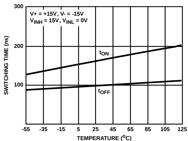
FIGURE 11. SWITCHING TIME vs TEMPERATURE, HI-304 THRU HI-307
