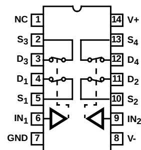
DUAL DPST HI-302 AND HI-306 (PDIP, CERDIP, SOIC) TOP VIEW
