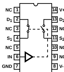
SPST HI-301 AND HI-305 TOP VIEWS
