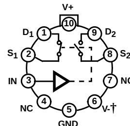
SPST HI-301 AND HI-305 TOP VIEWS
