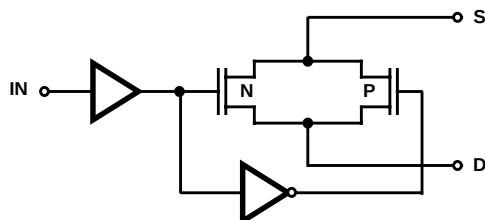
TYPICAL SWITCH HI-300 SERIES
