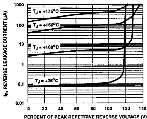
FIGURE 4. TYPICAL REVERSE LEAKAGE CURRENT CHARACTERISTICS
