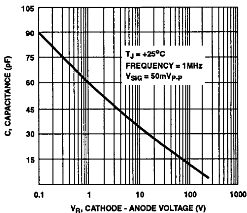
FIGURE 6. TYPICAL JUNCTION CAPACITANCE CHARACTERISTIC
