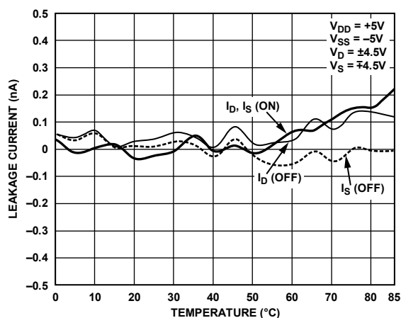
Figure 9. Leakage Currents vs. Temperature (Dual Supply)
