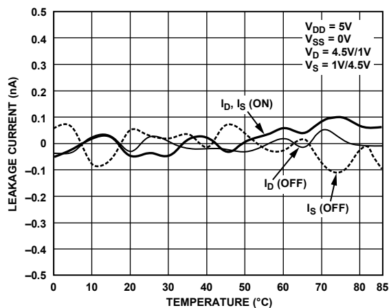
Figure 10. Leakage Currents vs. Temperature (Single Supply)
