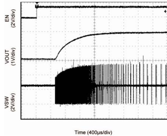
Start-Up Waveform
