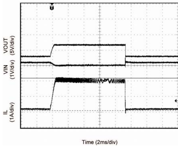
Current Limit
