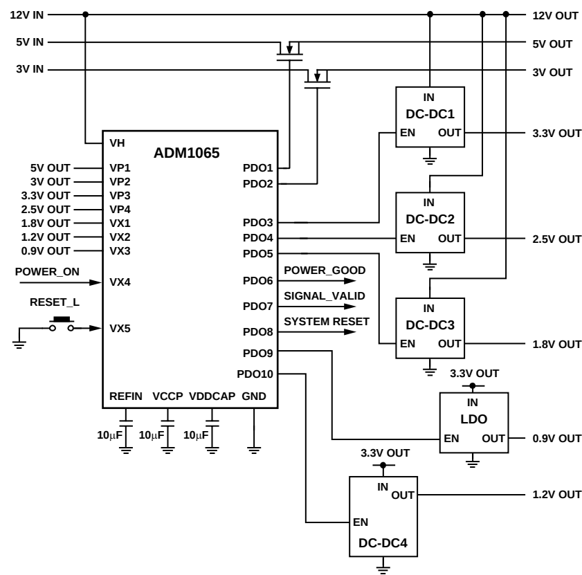
Figure 24. Applications Diagram
