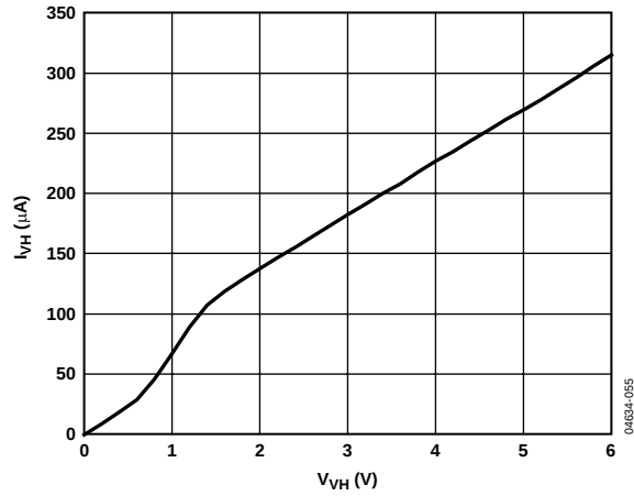
Figure 10. I VH vs. V VH (VH Not as Supply)
