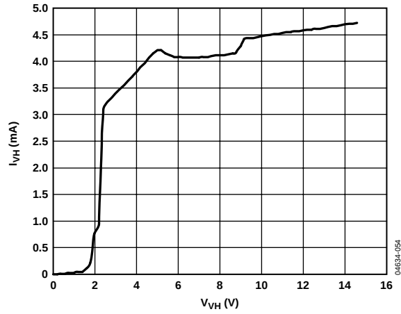
Figure 9. I VH vs. V VH (VH as Supply)
