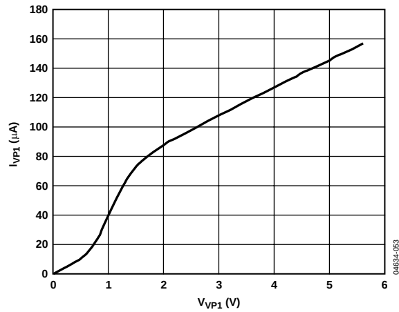
Figure 8. I VP1 vs. V VP1 (VP1 Not as Supply)
