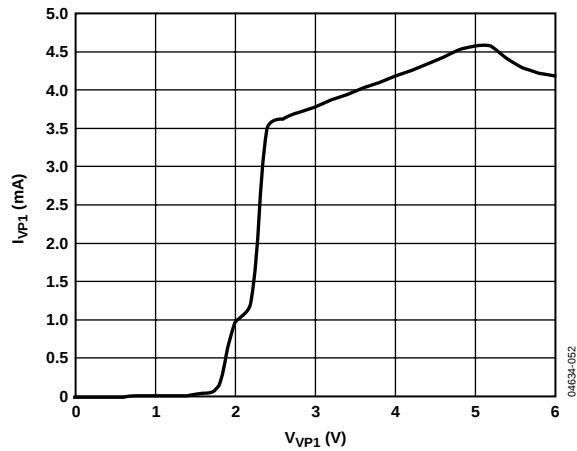
Figure 7. I VP1 vs. V VP1 (VP1 as Supply)
