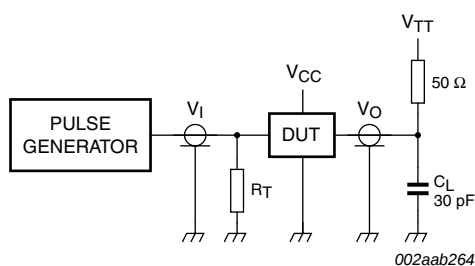
Fig 12. Load circuit for B outputs
