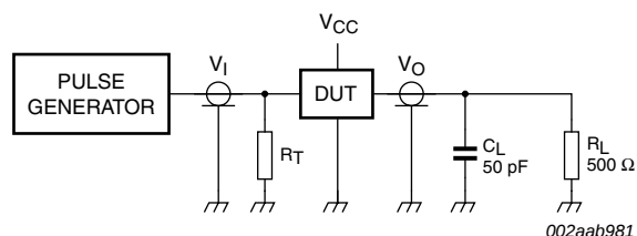
Fig 11. Load circuit for A outputs (9AO)
