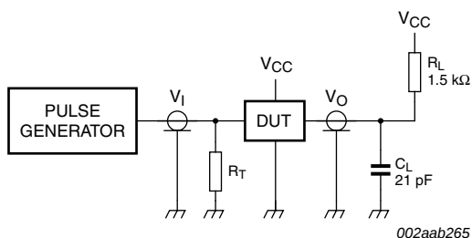
Fig 13. Load circuit for open-drain LVTTL I/O and open-drain outputs
