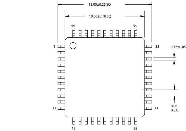
Figure 9. 44-Lead Thin Plastic Quad Flat Pack A44
