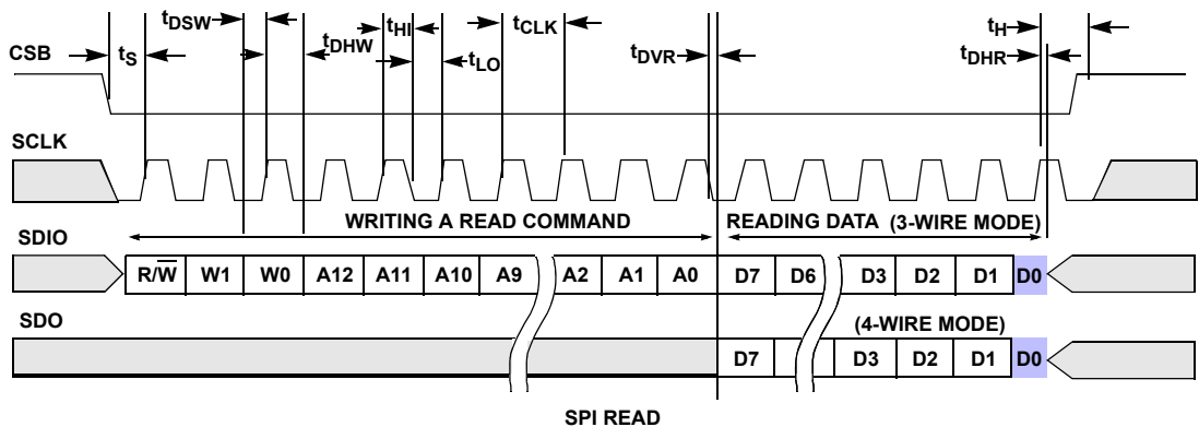
FIGURE 36. SPI READ
