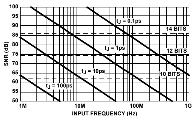
FIGURE 30. SNR vs CLOCK JITTER
