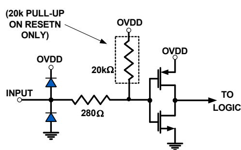
FIGURE 44. DIGITAL INPUTS
