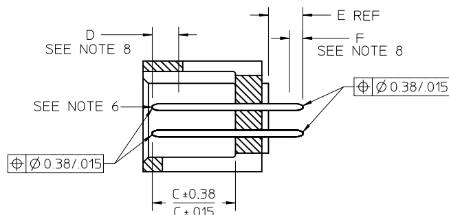
SECTION Y-Y
