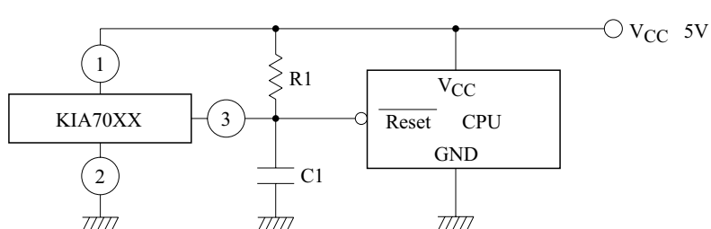
(2) CPU RESETTING
