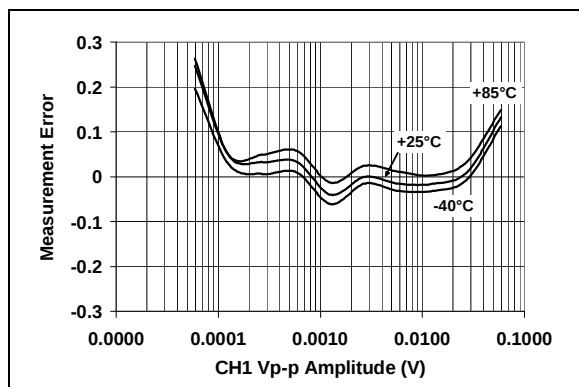
FIGURE 2-18: Measurement Error with External V_{REF} ( G = 8 ).
