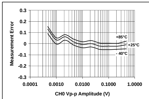
FIGURE 2-17: Measurement Error with External V_{REF} ( G = 1 ).
