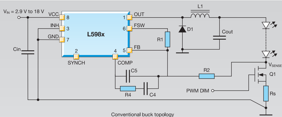
Conventional buck topology
