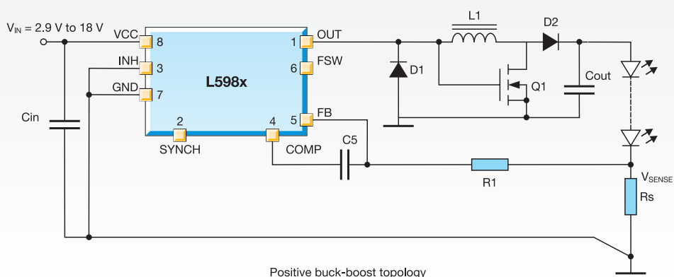
Positive buck-boost topology
