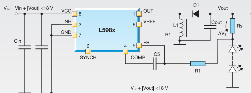
Inverting buck-boost topology
