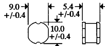
Terminal Dimensions
