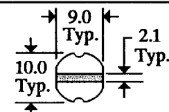
Terminal Dimensions
