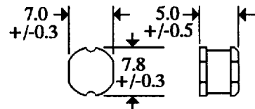
Terminal Dimensions
