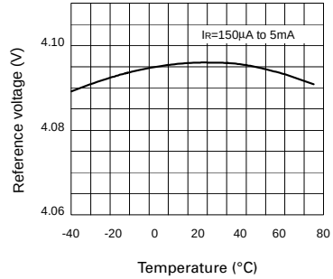
Temperature Drift
