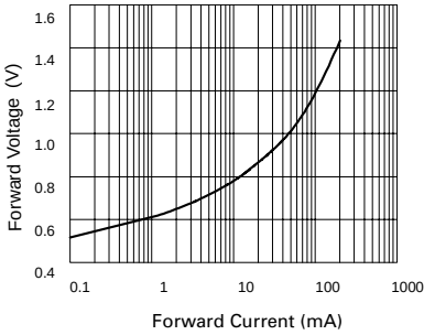
Forward Characteristics
