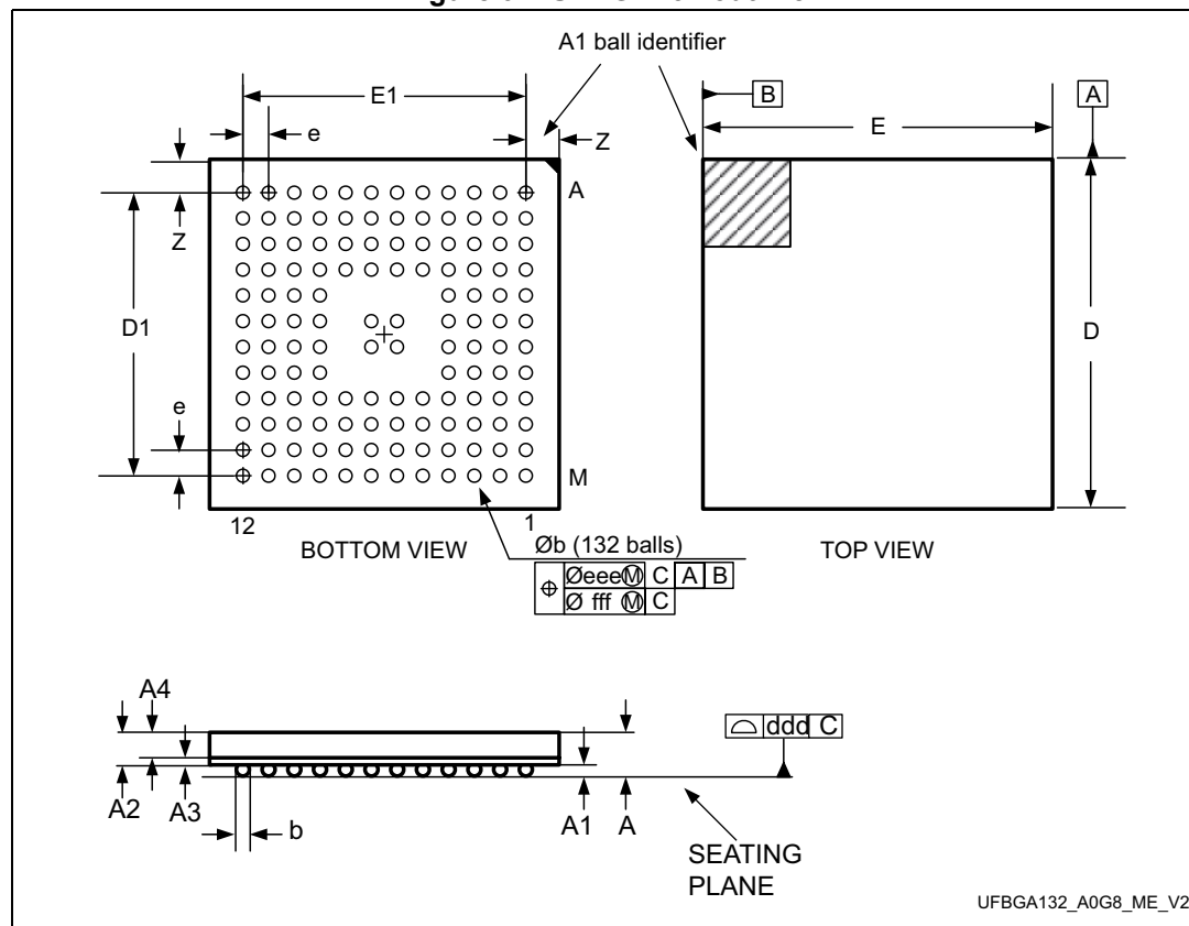
Figure 91. UFBGA132 outline
