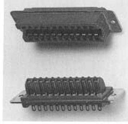
26-4100-XXP Plug 26-4200-XXS Receptacle
