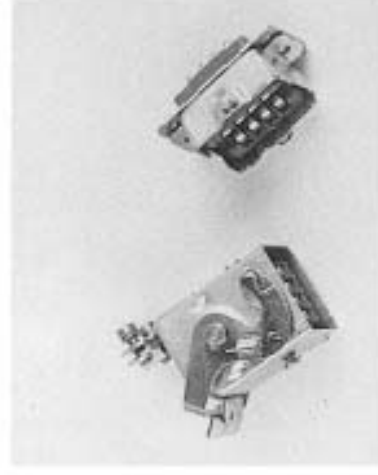
26-4301-XXS or 26-4301-XXP Plug
