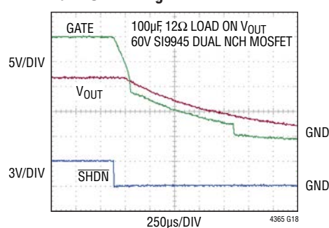
Turn-Off Timing
