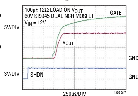
Turn-On Timing
