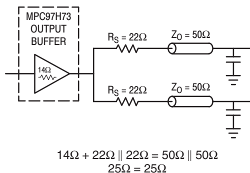
Figure 14. Optimized Dual Line Termination
