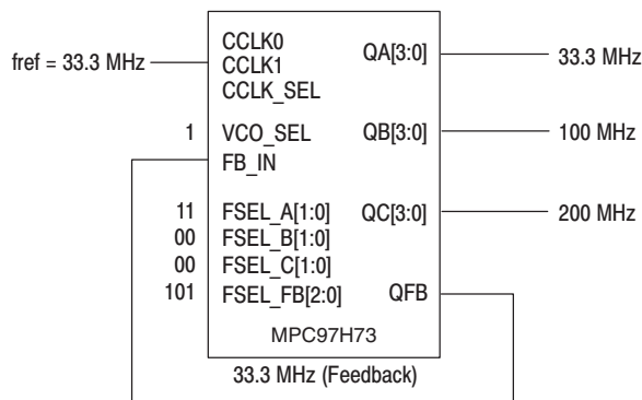
Figure 3. Example Configuration
