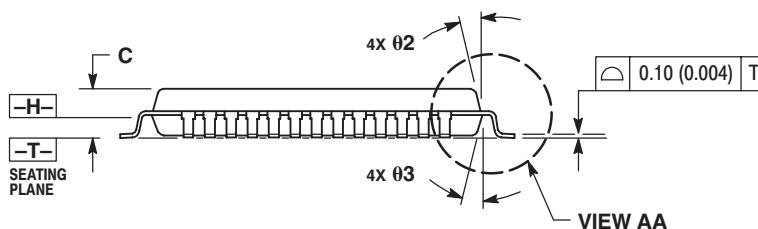
VIEW AA
