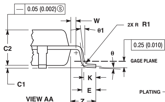
VIEW AA
