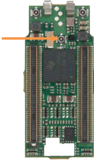
Figure 8.5: GPS Antenna Connector on DM3730 Torpedo + Wireless SOM
