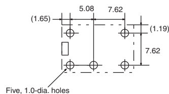
Mounting Holes (Bottom View) Tolerance: \pm 0.1
