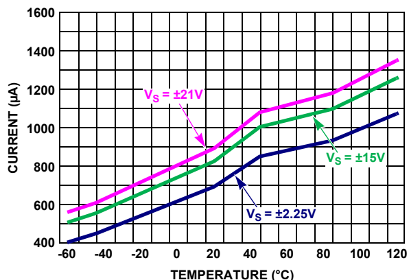
FIGURE 25. ISL28118M SUPPLY CURRENT vs TEMPERATURE vs SUPPLY VOLTAGE
