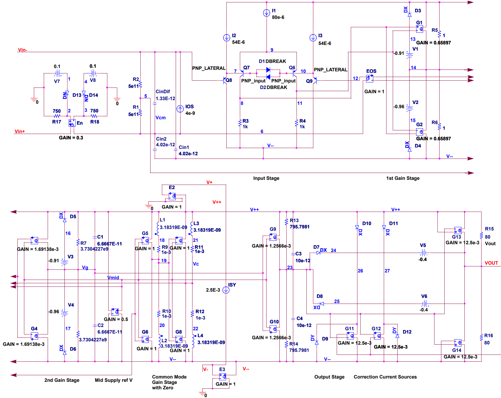
FIGURE 50. SPICE SCHEMATIC
