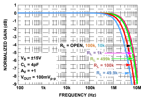
FIGURE 59. SIMULATED GAIN vs FREQUENCY vs R_L
