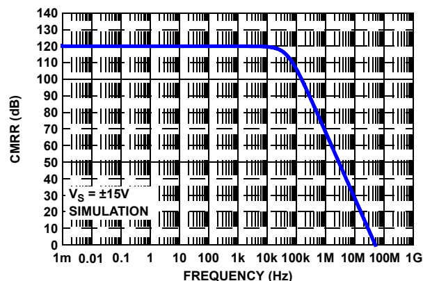
FIGURE 61. SIMULATED CMRR vs FREQUENCY
