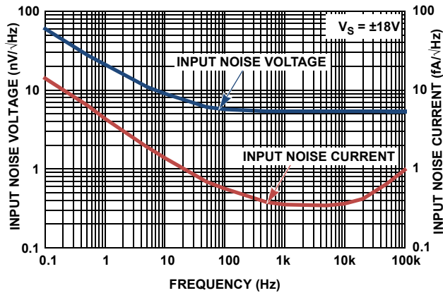
FIGURE 52. CHARACTERIZED INPUT NOISE VOLTAGE
