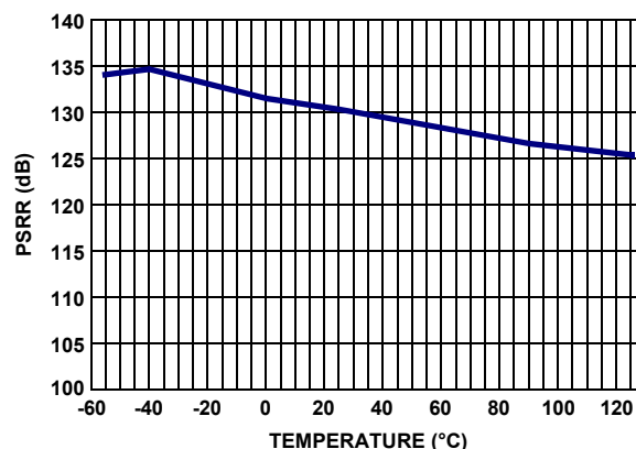
FIGURE 12. PSRR vs TEMPERATURE, V_S = \pm 15V
