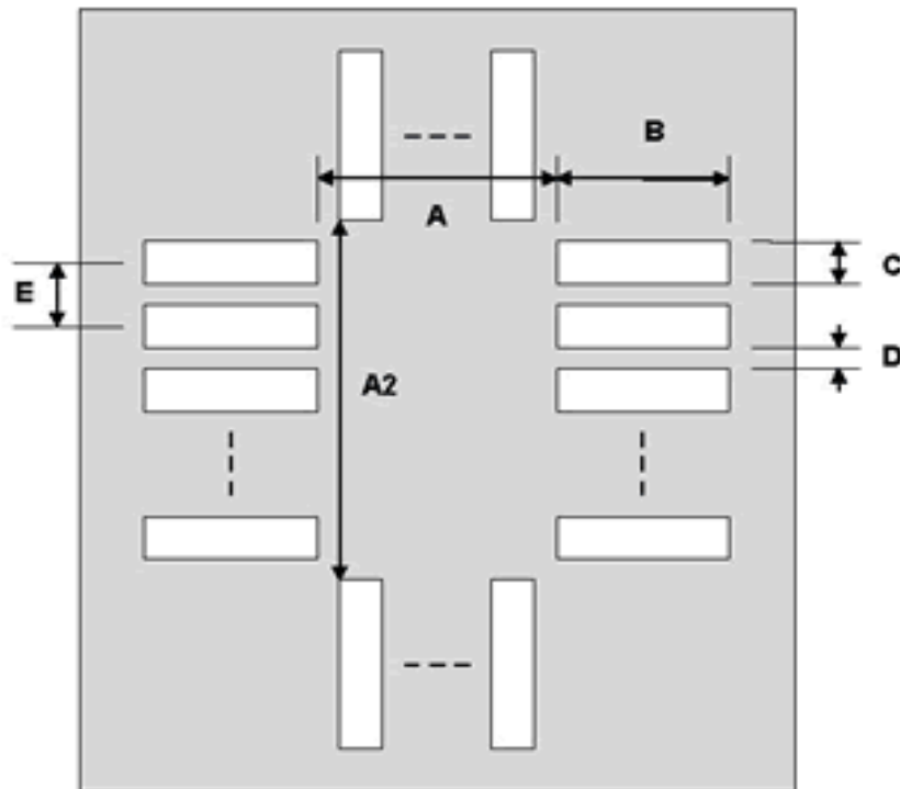
Top View (SMT Footprint)
