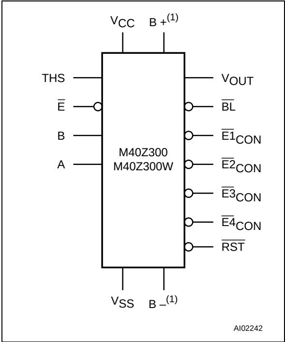
Figure 3. Logic Diagram
