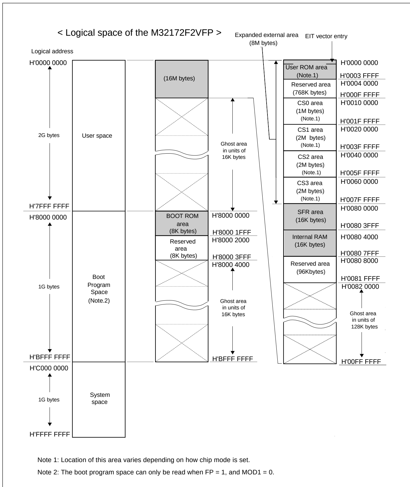
Figure 3: Address Space of the M32172F2VFP
