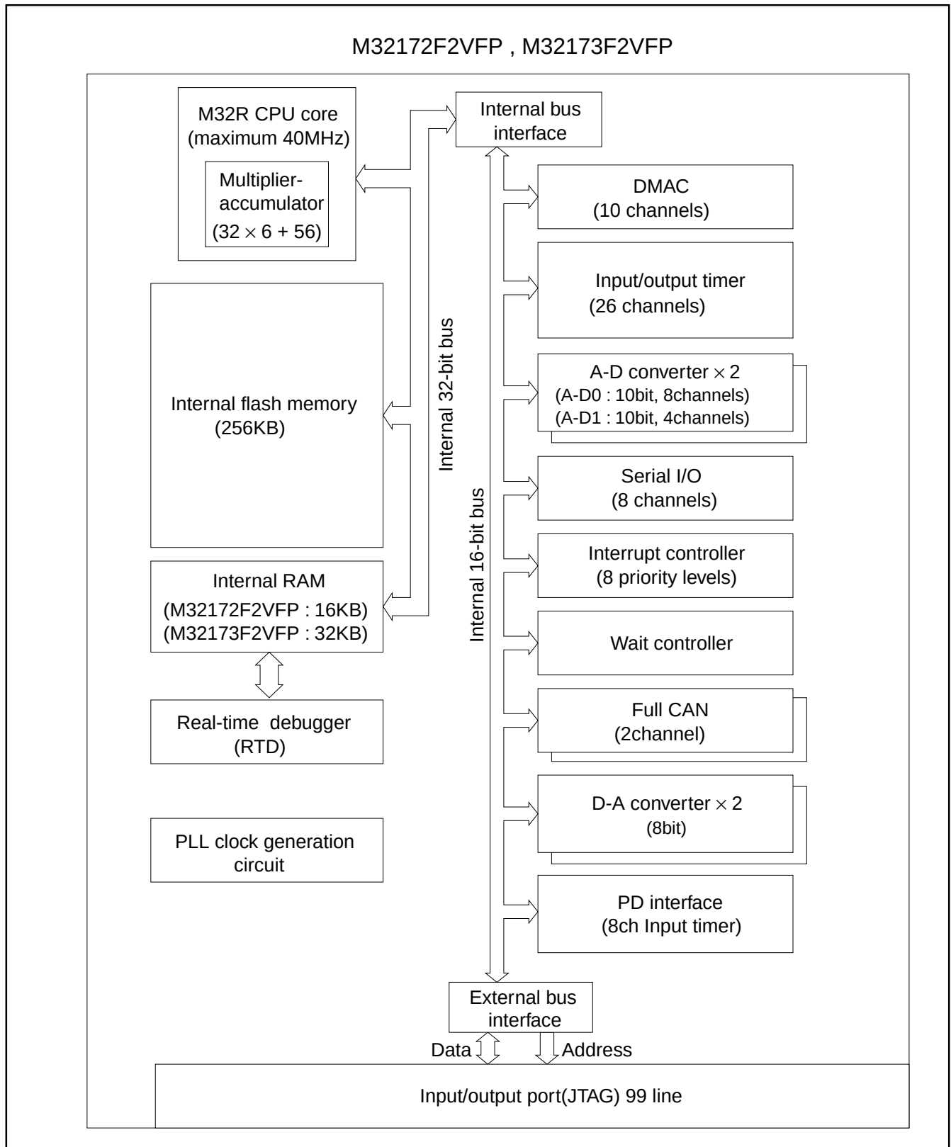
Fig.1 Block diagram
