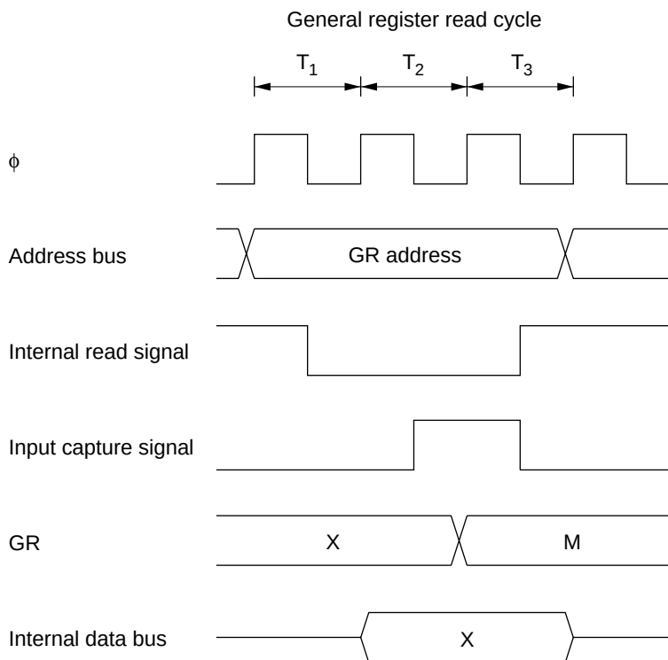
Figure 10.66 Contention between General Register Read and Input Capture
