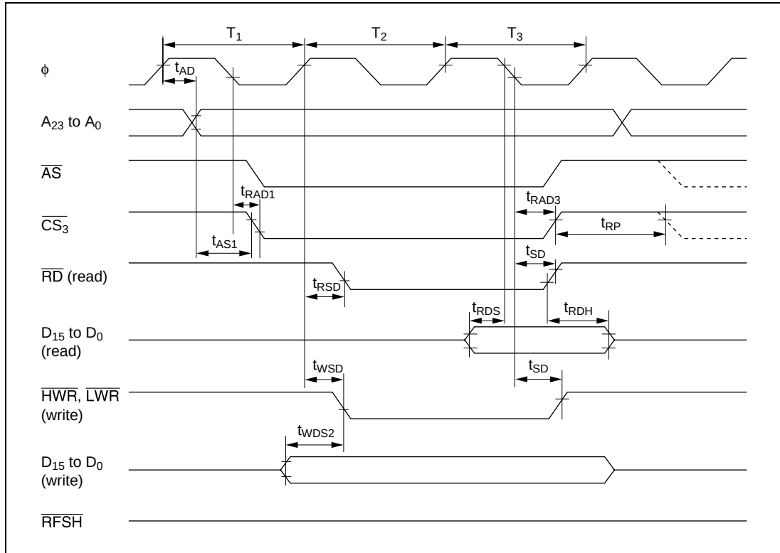
Figure 22.16 PSRAM Bus Timing (Read/Write): Three-State Access
