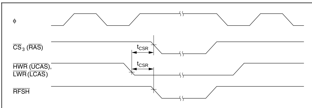
Figure 22.15 DRAM Bus Timing (Self-Refresh Mode) — \overline{2CAS} Mode —
