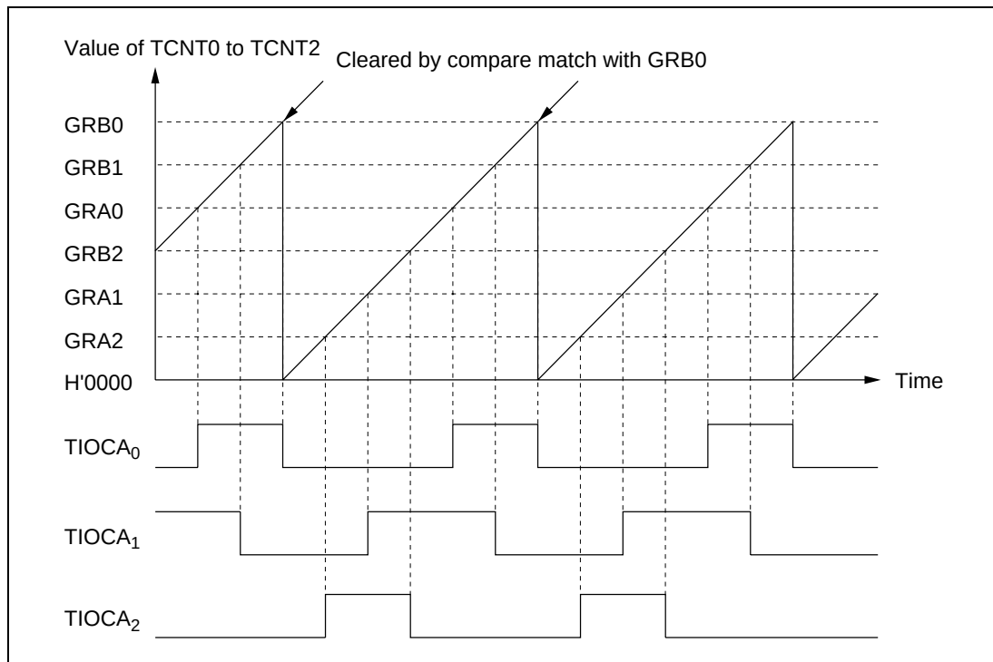
Figure 10.27 Synchronization (Example)
