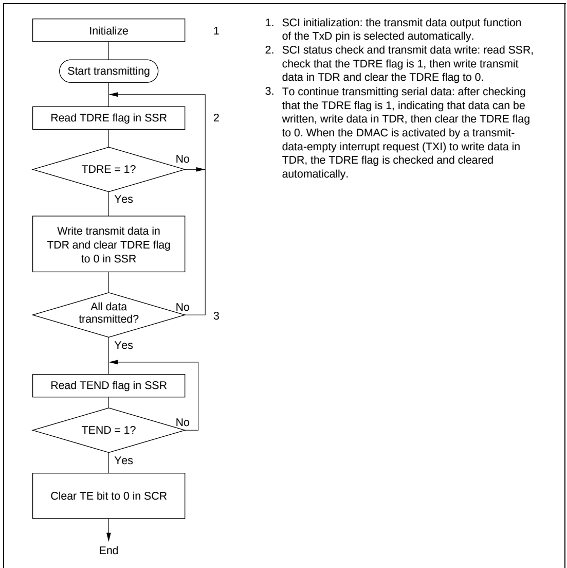
Figure 13.16 Sample Flowchart for Serial Transmitting
