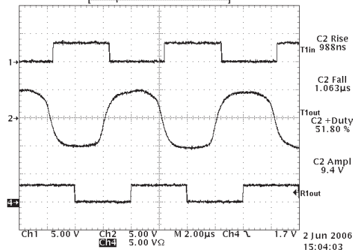
SP3244 Waveforms for 250kpbs Clock Rate RL=3kΩ CL=4700pF
