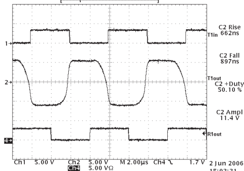
SP3244 Waveforms for 250kpbs Clock Rate RL=3kΩ CL=1000pF
