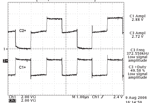
SP3244 C2+ Charge Pump Waveforms - Vcc=3.3V, All channels switching
