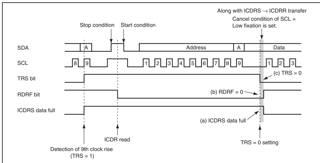
Figure 15.19 Notes on ICDR Reading with TRS = 1 Setting in Master Mode
