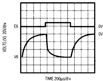
REGULATOR 7 TURN-ON TIME
