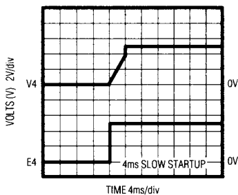
REGULATOR 4 TURN-ON TIME
