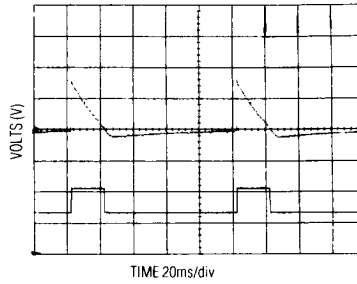
V2 LINE TRANSIENT RESPONSE
