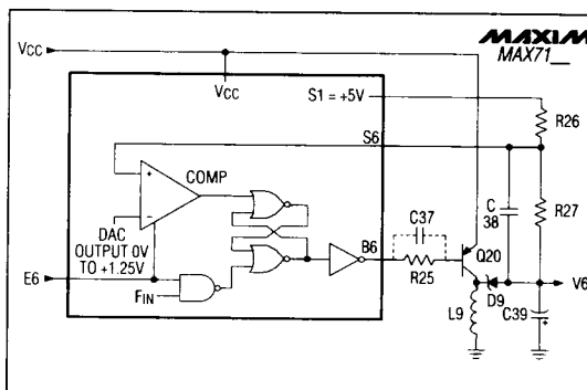
Figure 4. Functional Diagram and Circuit for DC-DC Converter V6
