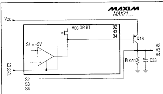
Figure 2. Functional Diagram and Circuit for Linear Regulators V2-V4
