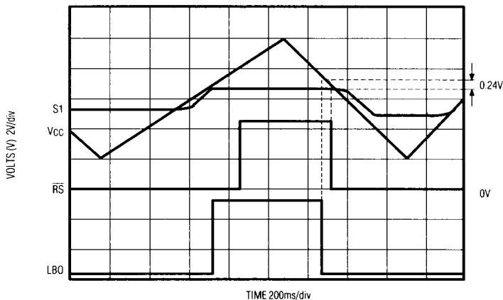
BACKUP-BATTERY SWITCHING AND WARNING FLAGS
