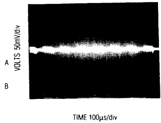
V5 LOAD-TRANSIENT RESPONSE
