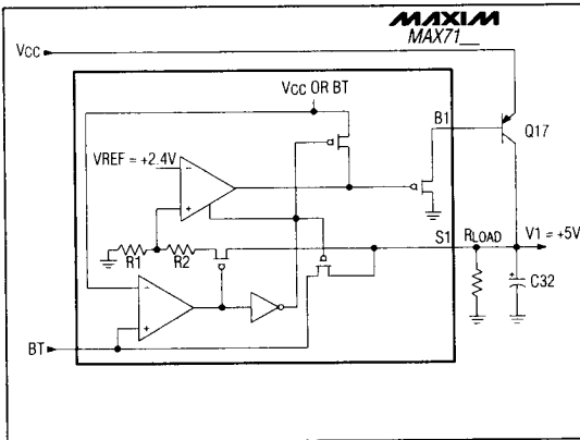
Figure 1. Functional Diagram and Circuit for Linear Regulator V1
