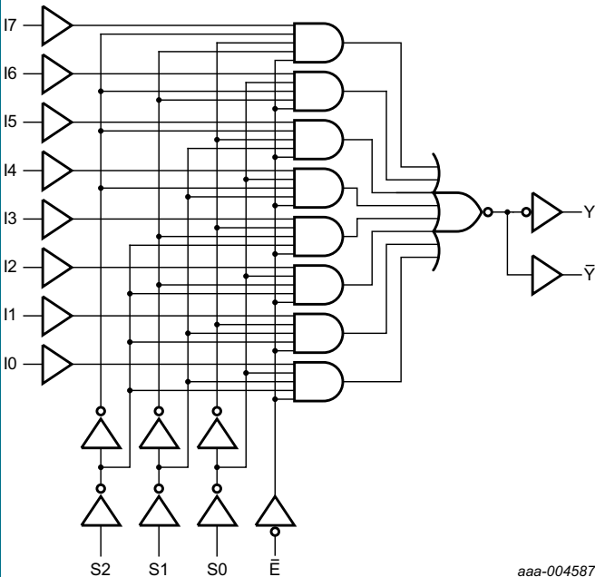
Fig 3. Logic diagram
