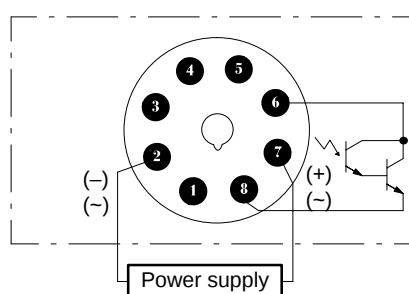
H3CR-A8S (Transistor Output)
