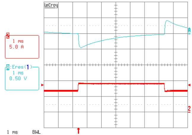
Figure L: Output voltage response to load current step-change (7.5A – 10A – 7.5A) at V_{in} = 48\text{ V} . Current slew rate: 0.1\text{ A}/\mu\text{s} . C_o = 220\text{ }\mu\text{F} aluminum electrolytic.
