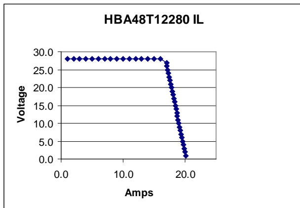
Figure P: Current limit of the HBA with V_{in} = 48\text{ VDC} .
