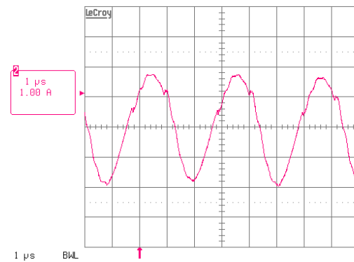
Figure V: Measurement of I_s with V_{cc} I_L = 12.5\ \text{Amps} , C_{out}=220\ \mu\text{F} , V_{in}=48\ \text{VDC} .
