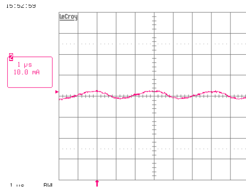
Figure U: Measurement of I_c with V_{cc} . I_L = 12.5\text{Amps} , C_{out} = 220\ \mu\text{F} , V_{in} = 48\ \text{VDC} .
