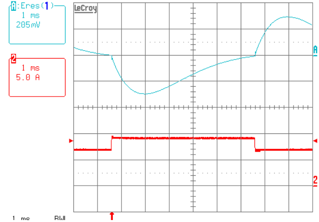
Figure M: Output voltage response to load current step-change (7.5A – 10A – 7.5A) at V_{in} = 48\text{ V} . Current slew rate: 1.0\text{ A}/\mu\text{s} . C_o = 4700\text{ }\mu\text{F} aluminum electrolytic.
