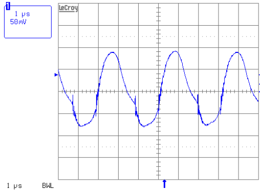
Figure N: Output Ripple Voltage, I_L=12.5\text{Amps} , C_{out}=220\ \mu\text{F} , V_{in}=48\text{ VDC} .
