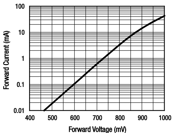
Figure 4. DC Characteristic
