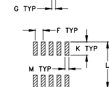
SUGGESTED LAYOUT FOR PCB LAND PATTERN
