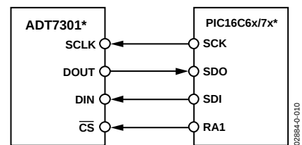
Figure 17. ADT7301-to-PIC16C6x/7x Interface
