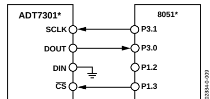
Figure 16. ADT7301 to 8051 Interface
