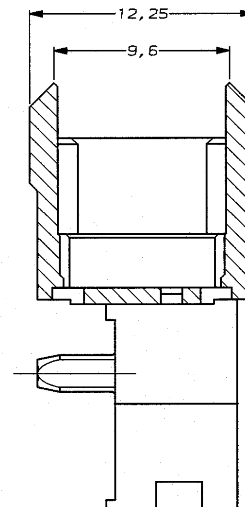
SECTION B-B
