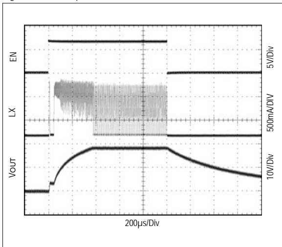
Figure 19. Startup Waveform
