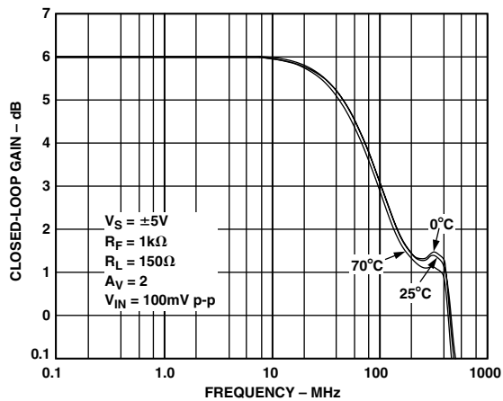
TPC 2. Frequency Response Over Temperature; V_S = \pm 5\text{ V}
