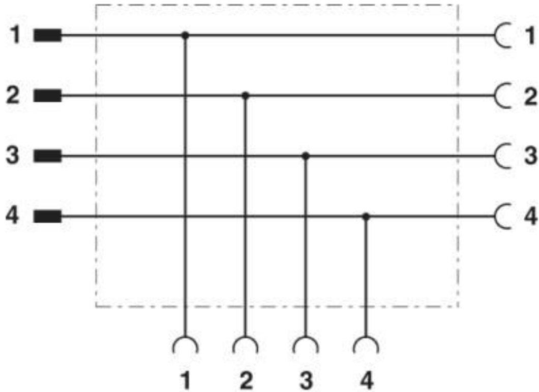
Contact assignment of the 7/8" T-distributor
