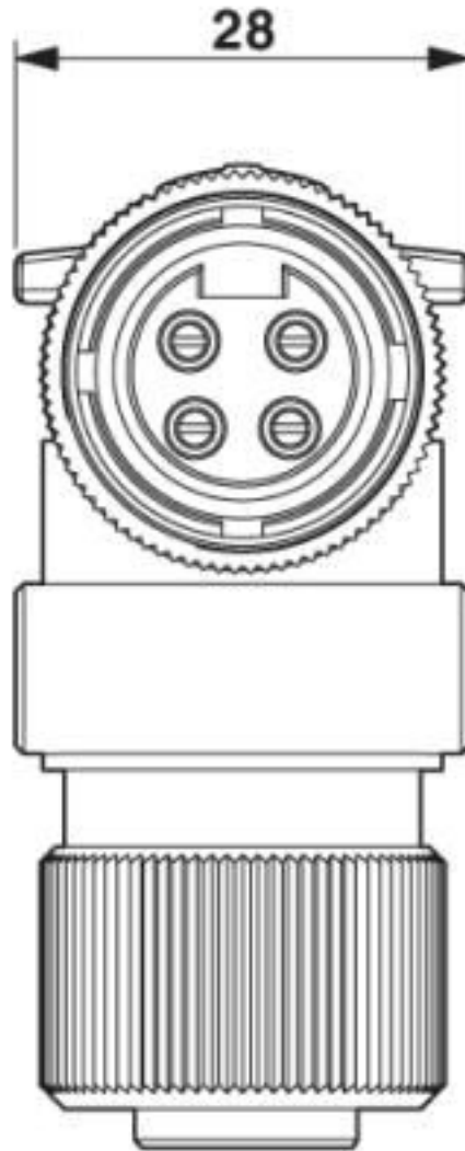
Dimensional drawing
