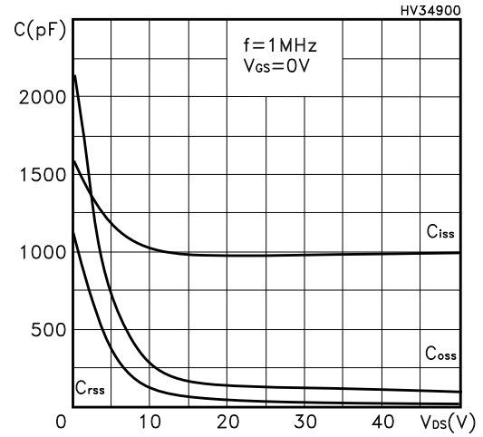
Figure 8. Capacitance variations
