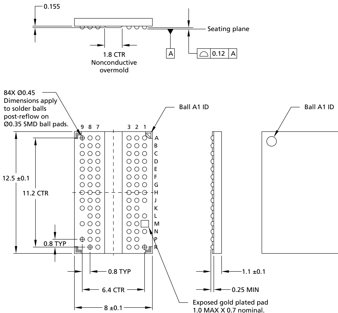
Figure 8: 84-Ball FBGA Package (8mm x 12.5mm) – x16
