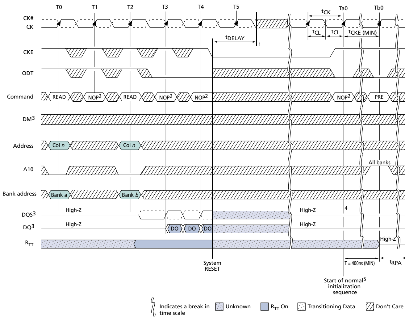
Figure 79: RESET Function
