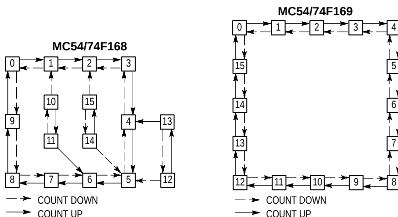
STATE DIAGRAMS
