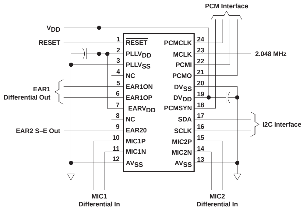
Figure 11. Typical EVM Interface to Support Circuitry
