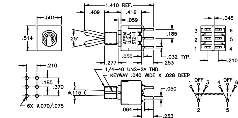
DOUBLE POLE
