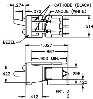
J95—TWO LED's
