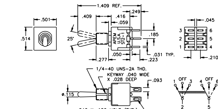
DOUBLE POLE
