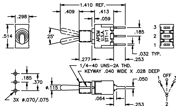
SINGLE POLE
