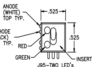
J95—TWO LED's
