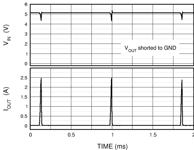
Over Current Retry Performance
